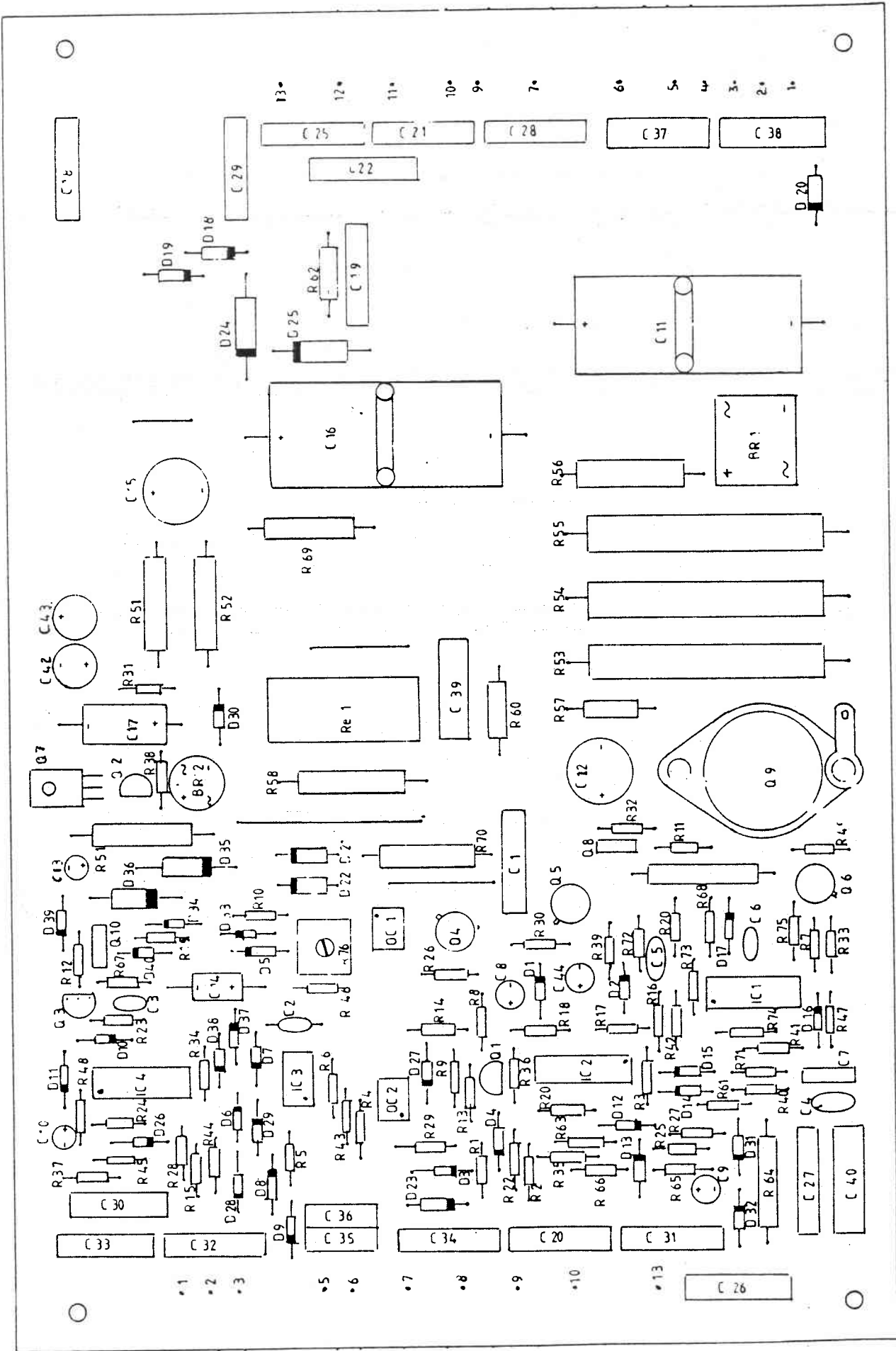
ACDC205 PCB 2 Board Layout
